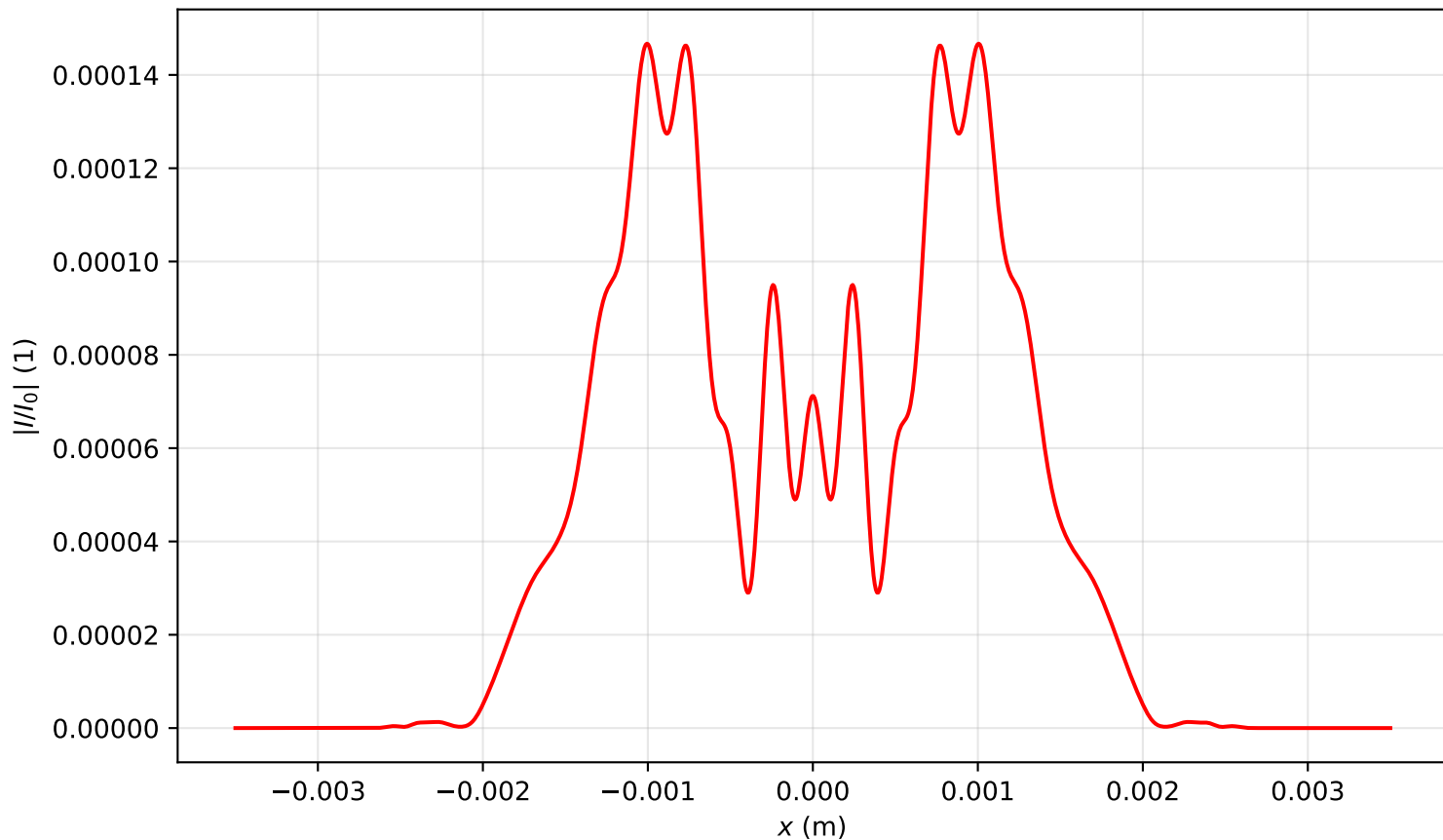
Intensity profile I(x, y = 0, z = 1.513)/I_0 , P_{in}=6.0P_{cr} , artificial time
